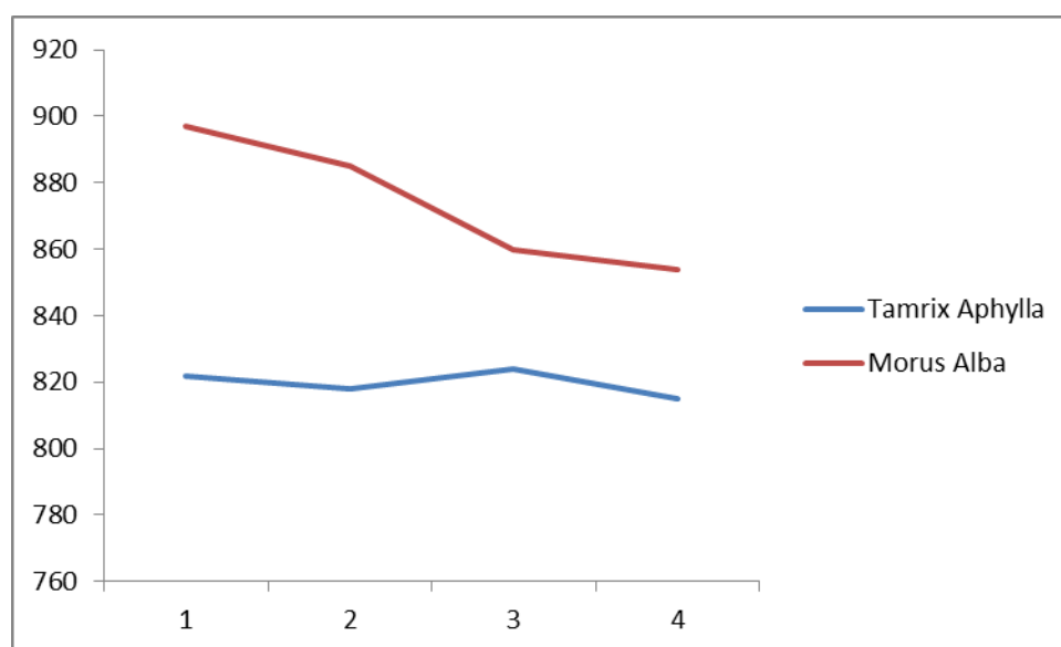
Figure 13: Variation in Density of Board Samples of Tamrix aphylla and Morus alba
