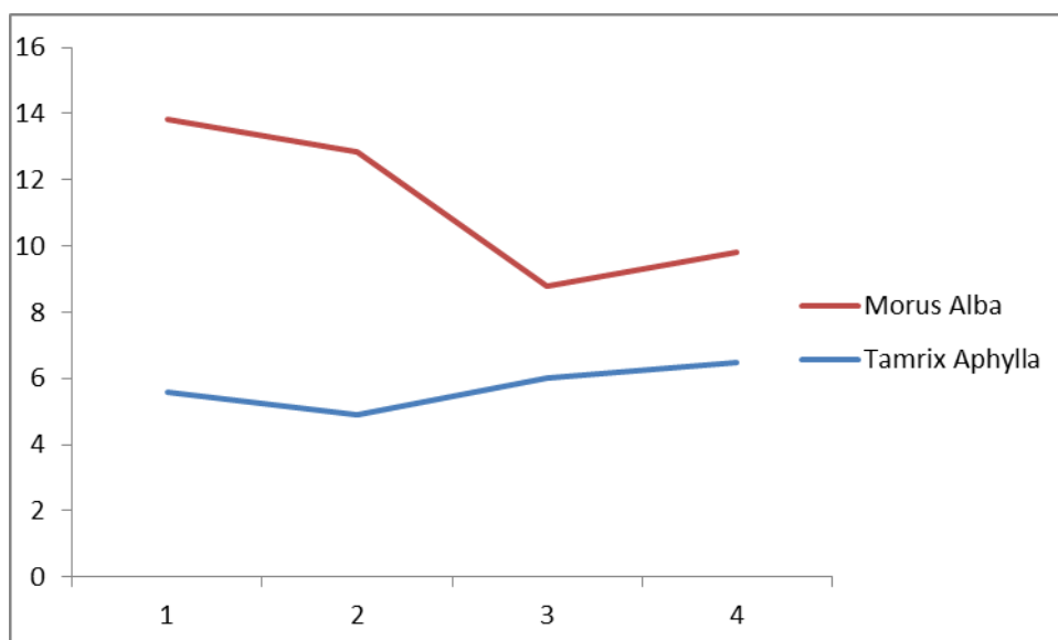
Figure 14: Variation of thickness swelling after 2 hrs.
