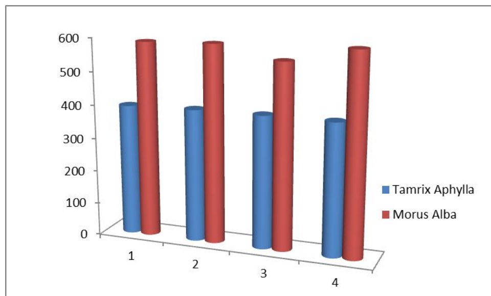
Figure 16: Variation in Modulus of Rupture of Board Samples
